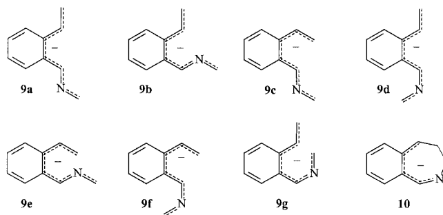
Figure 4. Conformations and configurations of the anions 9a–g and 10
