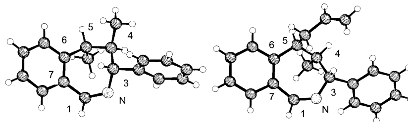
Figure 2. Molecular structure of compounds (3 R *,4 R *,5 R *)- 6b (left) and (3 R *,4 S *,5 S *)- 6d (right) in the solid state (X-ray analysis; only one enantiomer of each is shown)
