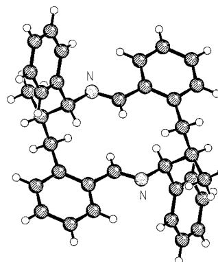
Figure 3. Molecular structure of the macrocycle 8 in the solid state (X-ray diffraction)
